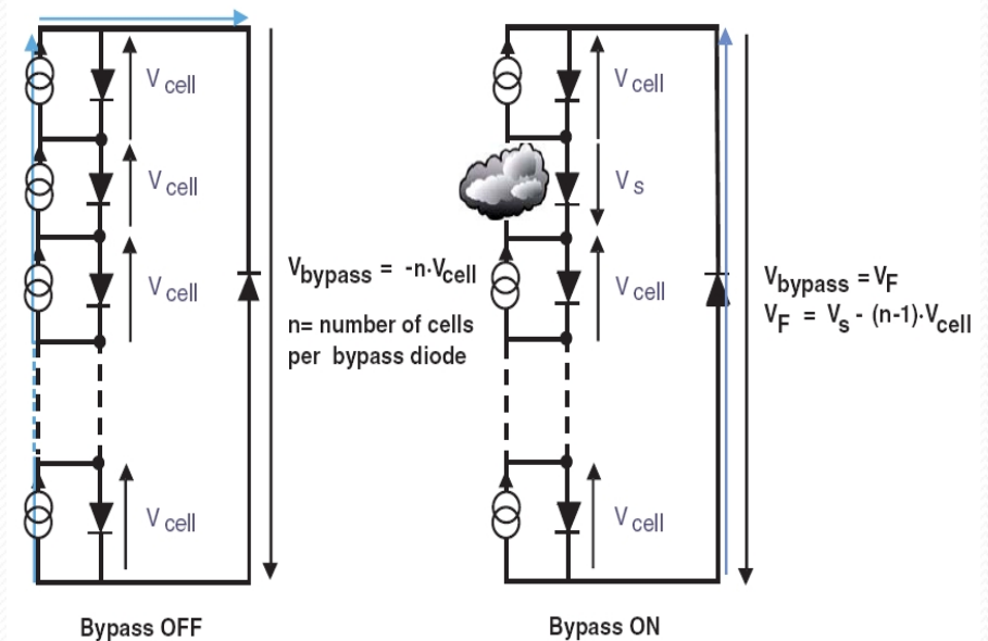
Bypass diode working phases
