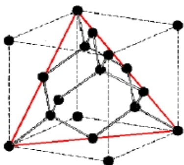
Unit cell of Si a=0.5431 nm
