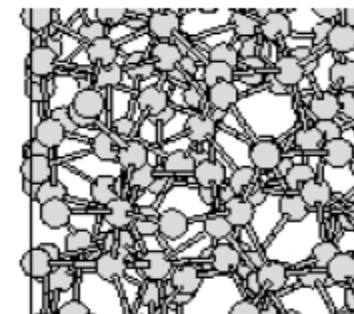
a-Si: H (very short range order in <1 nm regime)
